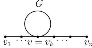
Figure 3: The graph P(n, k, G, v) .
