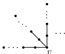
Figure 1: The d -pode R(c_1, \dots, c_d) .
