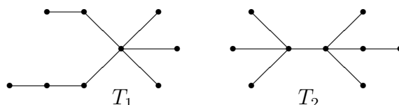
Figure 6: Two trees T_1, T_2 with Z(T_1) > Z(T_2) and \sigma(T_1) > \sigma(T_2) .
