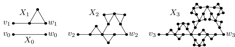
FIGURE 2. The Austria graphs X_0, X_1, X_2 , and X_3 .
