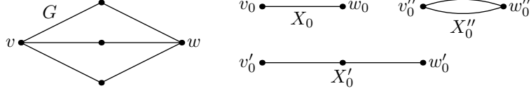
FIGURE 4. A model graph G and three initial graphs X_0, X'_0, X''_0 .
