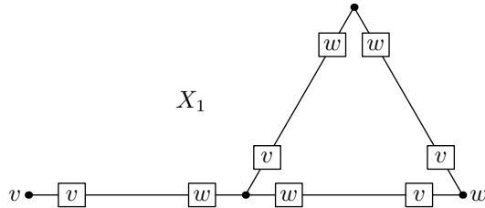
FIGURE 6. The first stage in the sequence of Austria graphs. Boxed labels indicate v -ends and w -ends of edges.
