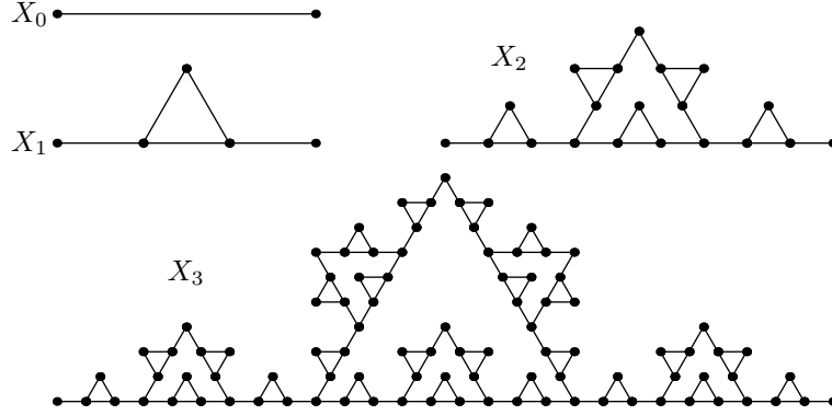
FIGURE 3. The finite modified Koch graphs X_0, X_1, X_2 , and X_3 .
