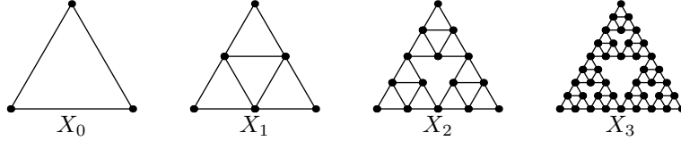
FIGURE 1. Finite Sierpiński graphs X_0, X_1, X_2, X_3 .
