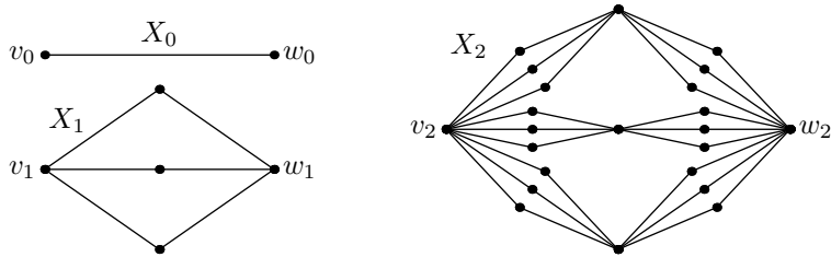
FIGURE 5. The graphs X_0, X_1, X_2 .
