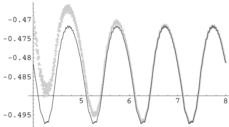
FIGURE 3. Fluctuation for (b, a, \Delta) = (5, 7, 23) and \eta = 30 : The gray dots are (S_{30}(N) - 1/5N \log_5 N)/N , the black line is \Phi_{30}(x) (approximated with 201 Fourier coefficients). The x -axis is scaled logarithmically (base 5).
