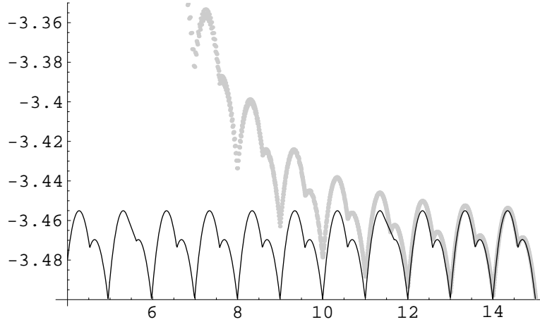
FIGURE 4. Fluctuation in the length for (b, a, \Delta) = (2, 1, 3) : The gray dots are (\sum_{n < N} \ell(n) - N \log_2 N)/N , the black line is \Phi(x) (approximated with 101 Fourier coefficients). The x -axis is scaled logarithmically (base 2).
