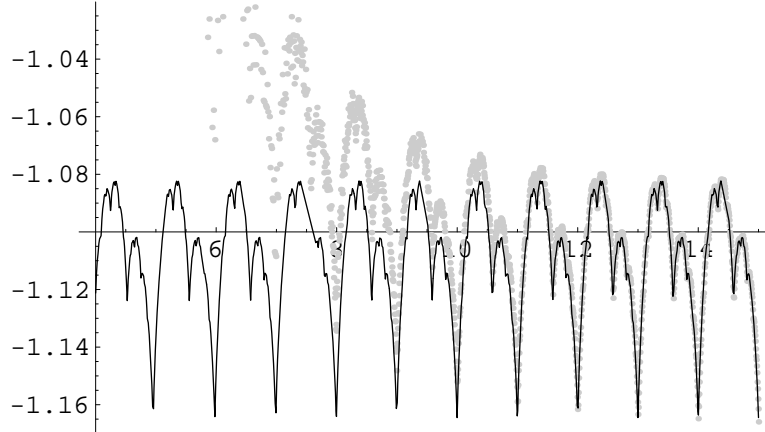
FIGURE 1. Fluctuation for (b, a, \Delta) = (2, 1, 3) and \eta = 1 : The gray dots are (S_1(N) - 1/2 N \log_2 N)/N , the black line is \Phi_1(x) (approximated with 101 Fourier coefficients). The x -axis is scaled logarithmically (base 2).
