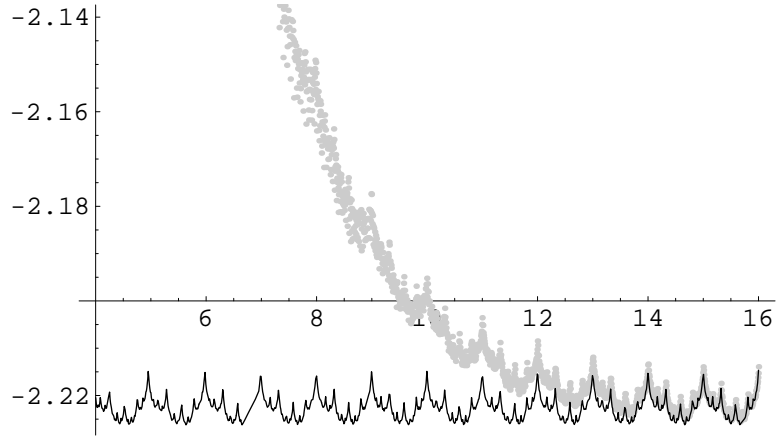
FIGURE 2. Fluctuation for (b, a, \Delta) = (2, 1, 7) and \eta = 8 : The gray dots are (S_8(N) - 1/2N \log_2 N)/N , the black line is \Phi_8(x) (approximated with 201 Fourier coefficients). The x -axis is scaled logarithmically (base 2).
